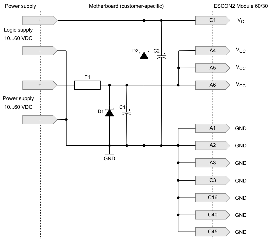
Figure 4-31 Wiring of logic supply
