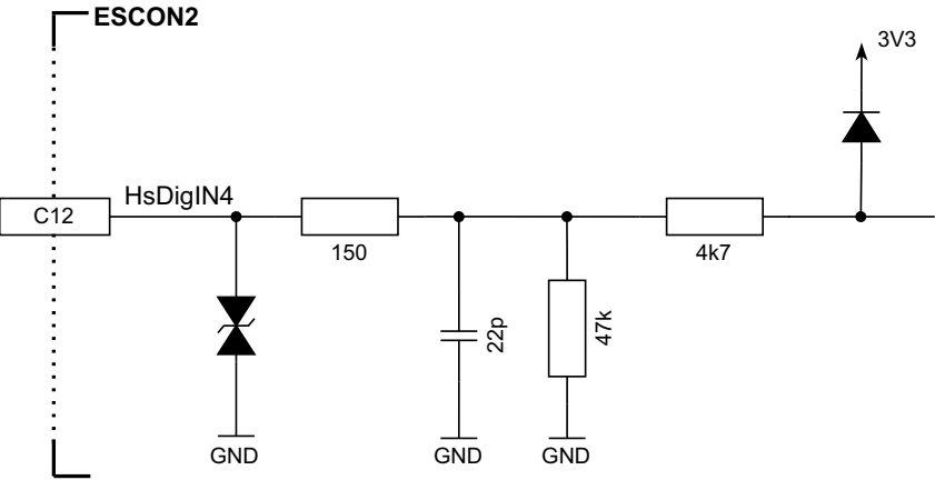
Figure 3-15 HsDigIN4 circuit “single-ended”
