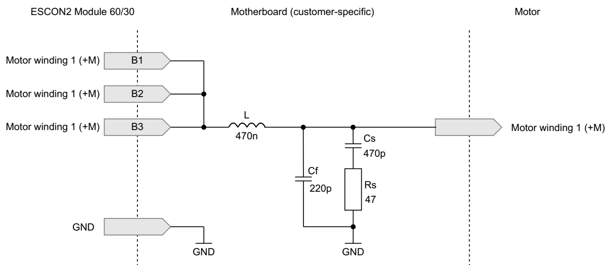
Figure 4-32 Wiring of motor winding 1 (analogously valid for motor winding 2 & 3)
