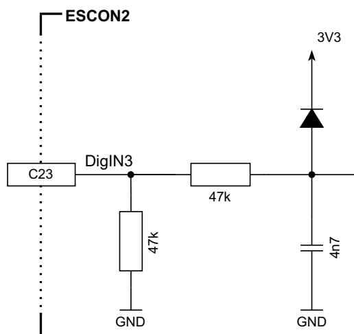
Figure 3-20 DigIN3 circuit (analogously valid for DigIN4)
