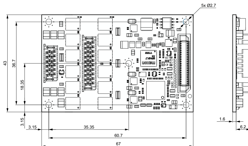
Figure 2-6 Dimensional drawing [mm]
