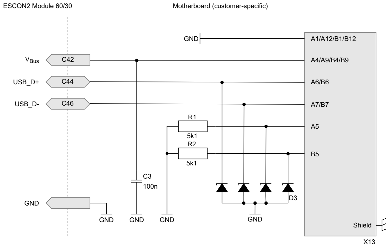
Figure 4-33 Wiring of USB-C connector
