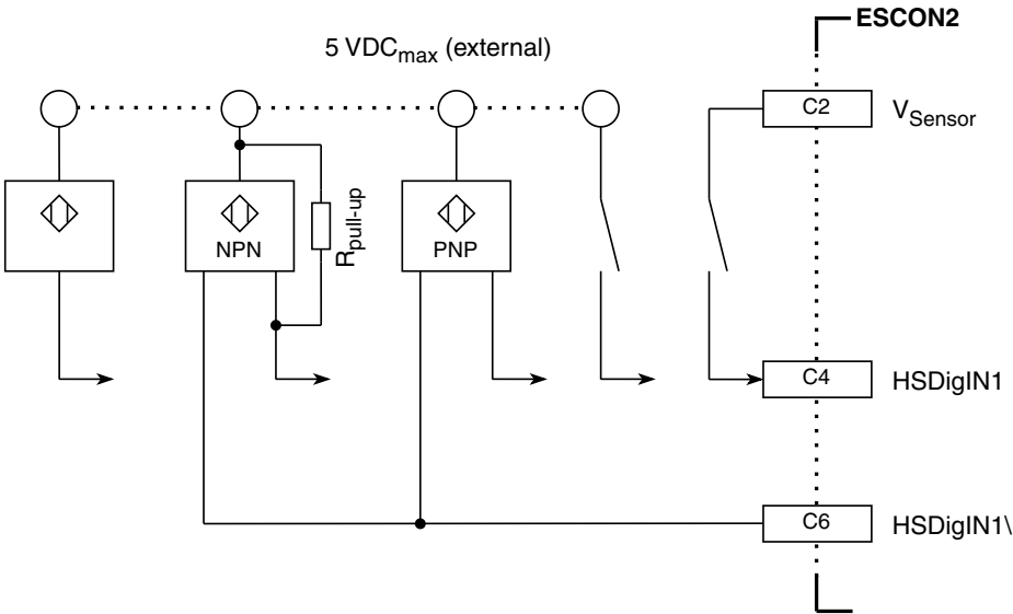
Figure 3-16 Wiring examples for proximity sensors and switches on HsDigIN1 (analogously valid for HsDigIN2)
