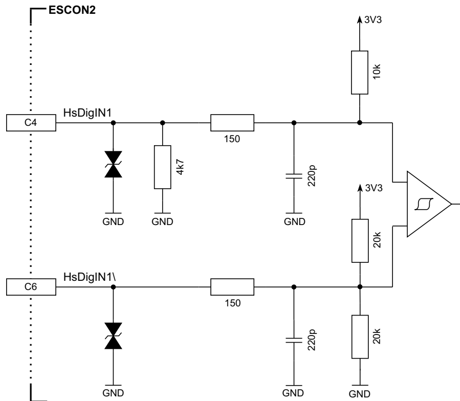
Figure 3-13 HsDigIN1 circuit “differential” (analogously valid for HsDigIN2)
