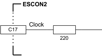
Figure 3-12 SSI absolute encoder clock output (analogously valid for BiSS C)
