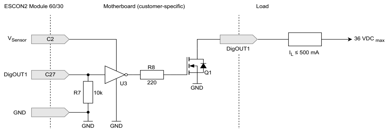
Figure 4-38 Wiring of digital output 1 load switch (analogously valid for digital output 2)
