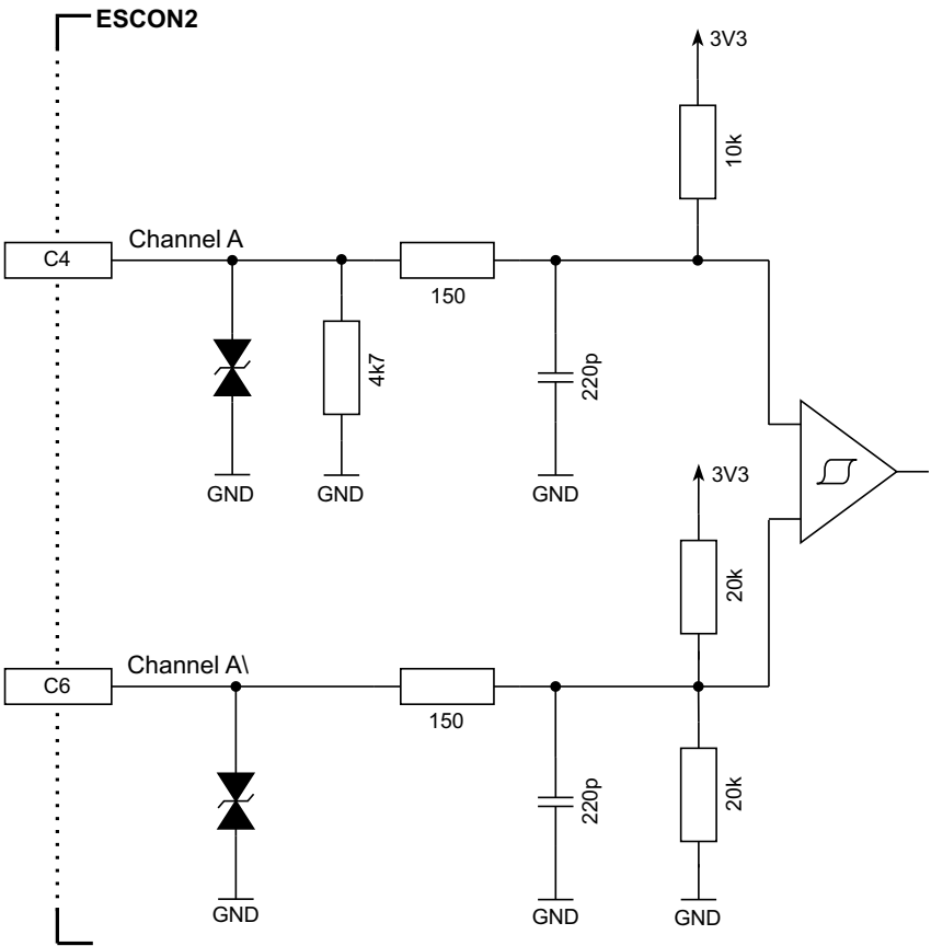
Figure 3-9 Digital incremental encoder input circuit Ch A “differential” (analogously valid for Ch B)
