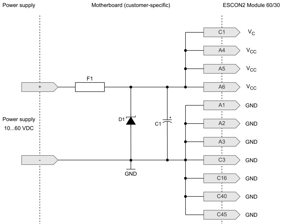
Figure 4-30 Wiring of power supply
