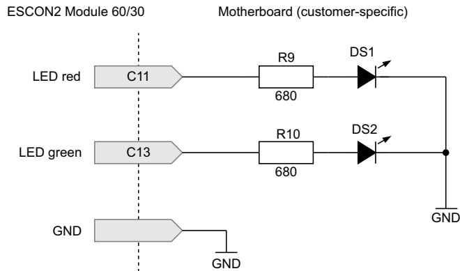
Figure 4-39 Wiring of LEDs for device status indication
