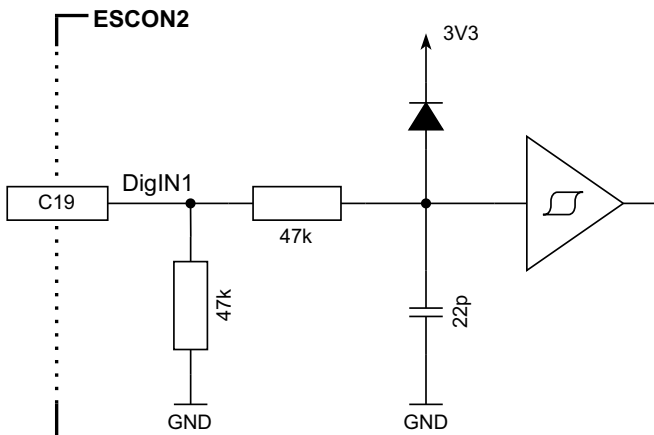
Figure 3-19 DigIN1 circuit (analogously valid for DigIN2)
