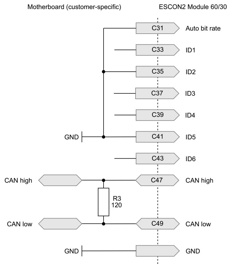
Figure 4-34 Wiring of CAN interface
