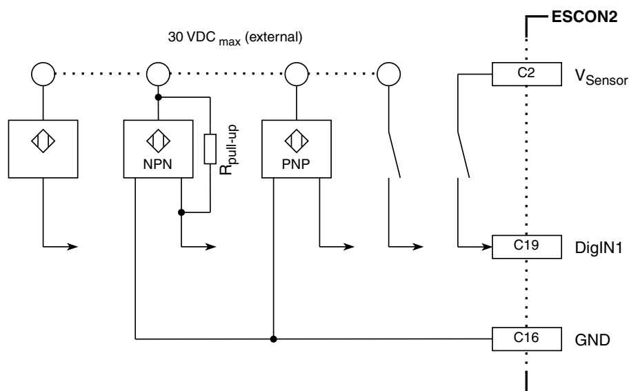
Figure 3-21 Wiring examples for proximity sensors and switches on DigIN1 (analogously valid for DigIN2...4)
