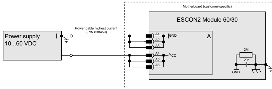
Figure 5-43 Power supply
