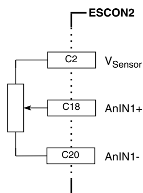
Figure 3-25 Wiring examples for a potentiometer on AnIN1 (analogously valid for AnIN2)
