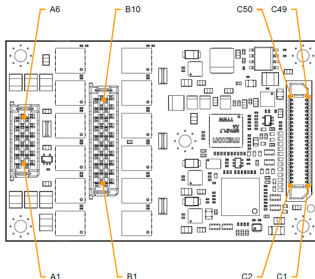
Figure 5-41 Interfaces – Designations and location
