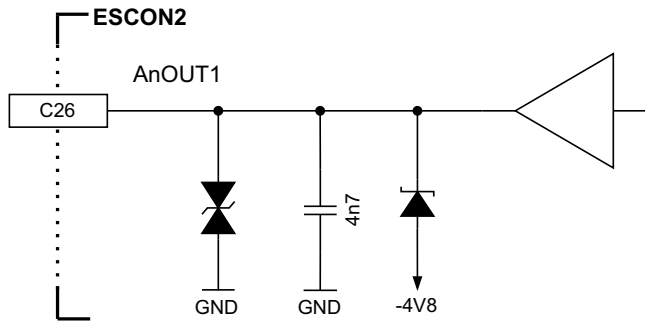
Figure 3-26 AnOUT1 circuit (analogously valid for AnOUT2)
