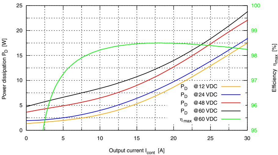
Figure 2-5 Power dissipation and efficiency
