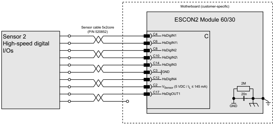
Figure 5-50 High-speed digital I/Os
