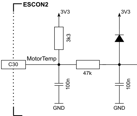
Figure 3-28 Motor temperature circuit
