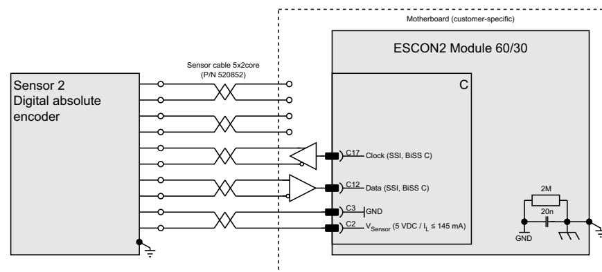
Figure 5-49 SSI / BiSS C unidirectional absolute encoder
