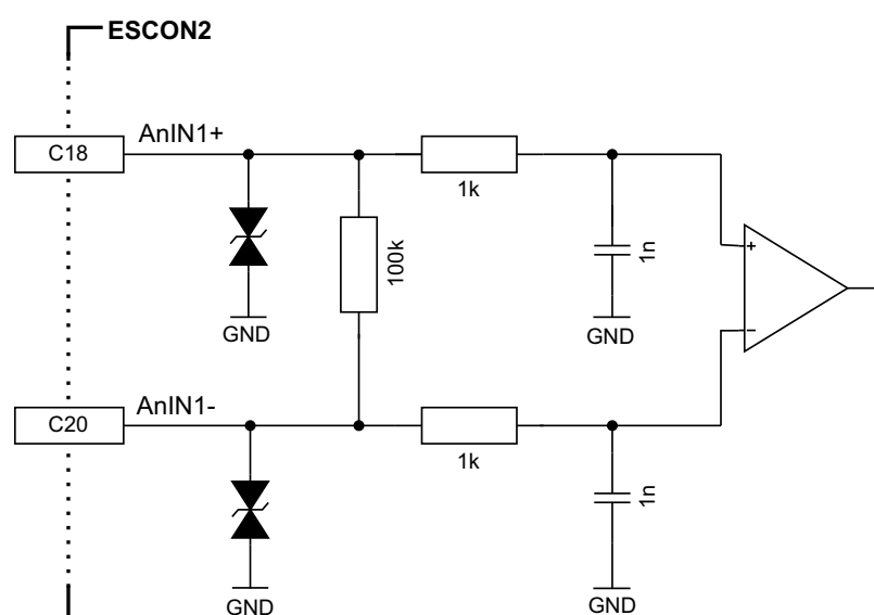
Figure 3-24 AnIN1 circuit (analogously valid for AnIN2)
