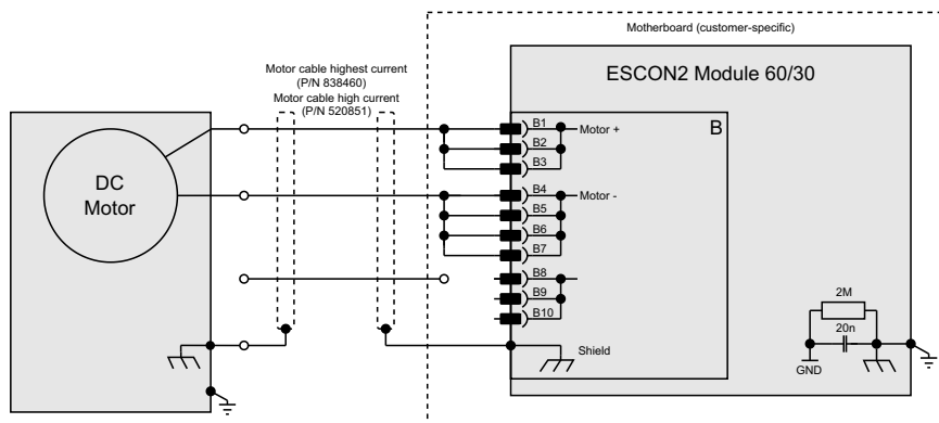
Figure 5-45 DC motor
