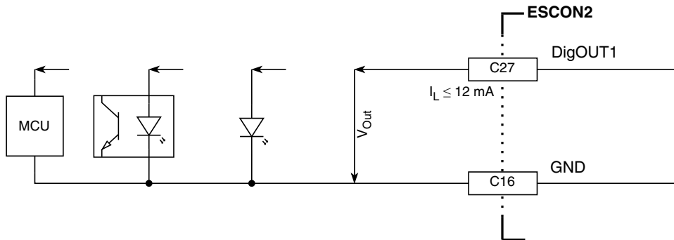
Figure 3-23 Wiring examples for "sourcing" on DigOUT1 (analogously valid for DigOUT2)
