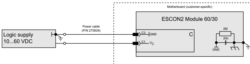
Figure 5-44 Logic supply
