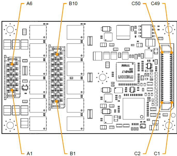
Figure 3-7 Pin assignment
