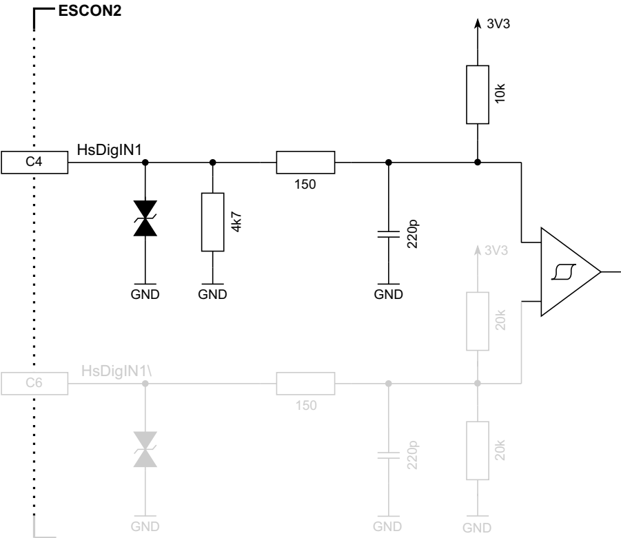
Figure 3-14 HsDigIN1 circuit “single-ended” (analogously valid for HsDigIN2...3)
