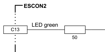
Figure 3-29 LED green circuit (analogously valid for LED red)
