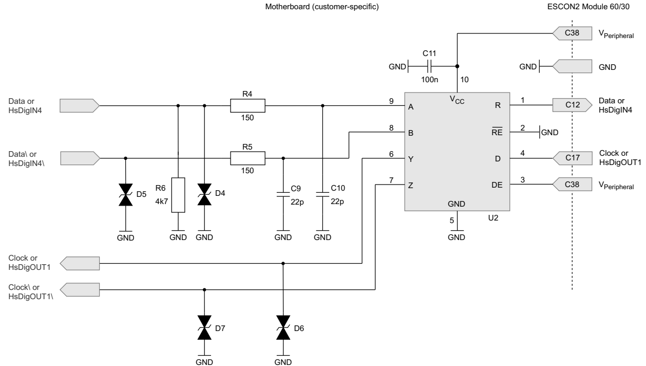
Figure 4-37 Wiring of RS422 transceiver
