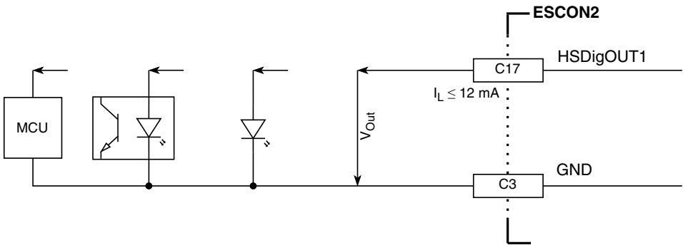
Figure 3-18 Wiring examples for "sourcing" on HsDigOUT1
