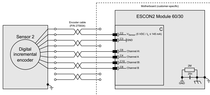
Figure 5-48 Digital incremental encoder
