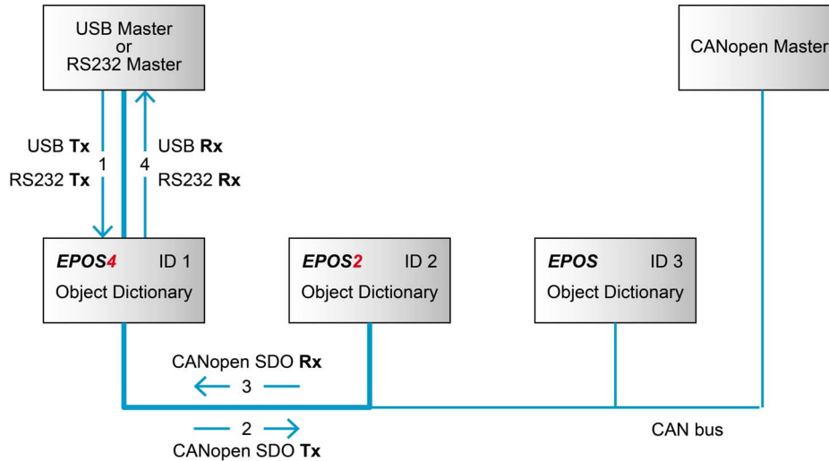
Figure 5-26 Gateway communication – Structure
