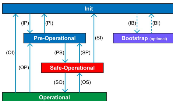
Figure 4-25 EtherCAT communication – ESM scheme
